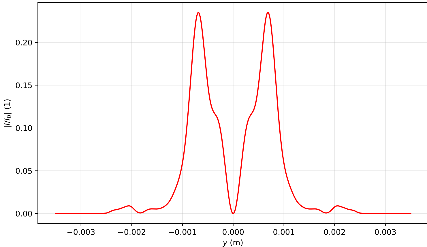
Intensity profile I(x=0, y, z=2.149)/I_0 , \text{Pin}=5.0\text{Pcr} , artificial time
